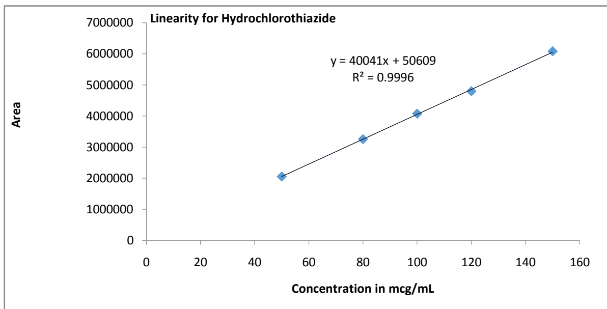
FIGURE: 4 Linearity of peak area at 280nm to corresponding concentration of HCT
