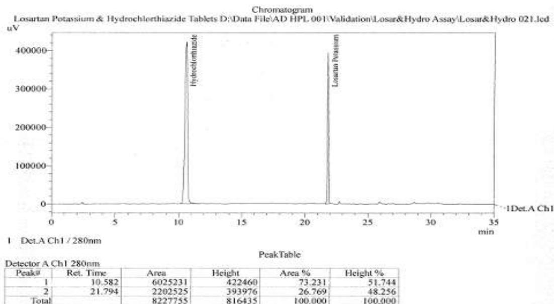
FIGURE 3:Chromatogram of losartan potassium and Hydrochlorthiazide
