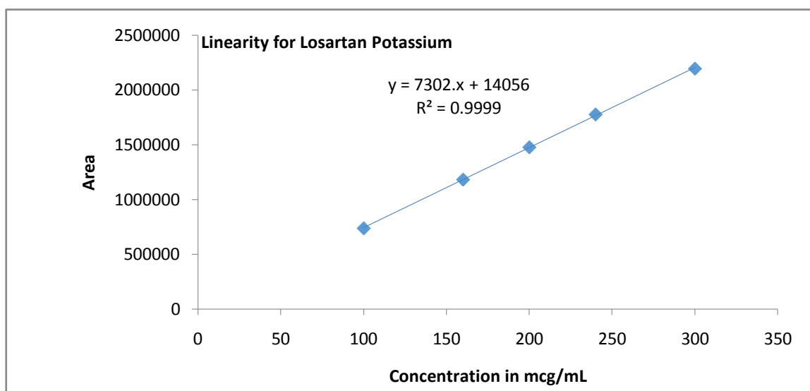
FIGURE: 5 Linearity of peak area at 280nm to corresponding concentration of LOS
